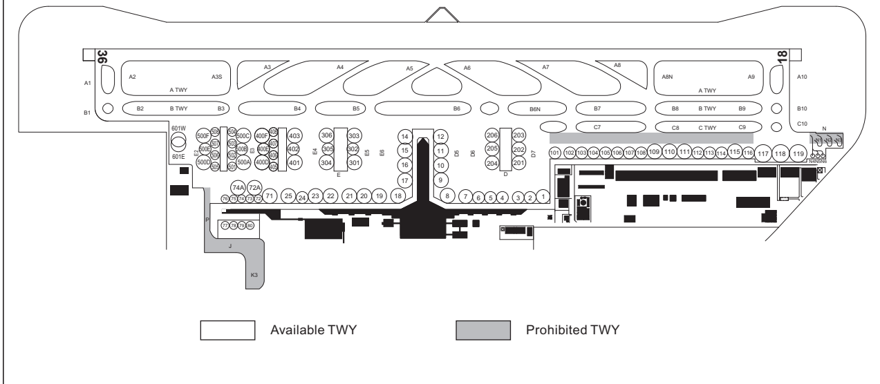
Taxiway routes available to the aircraft (65m<WS=<70m)
