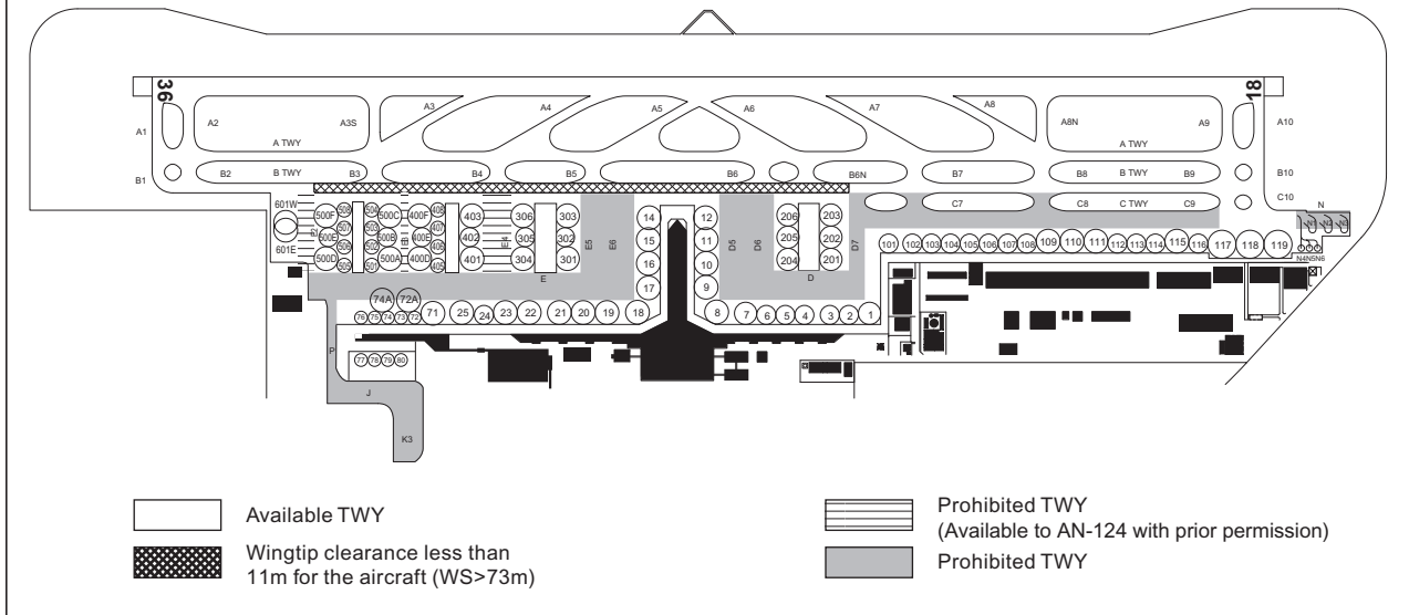
Taxiway routes available to the aircraft (70m<WS=<74m)
