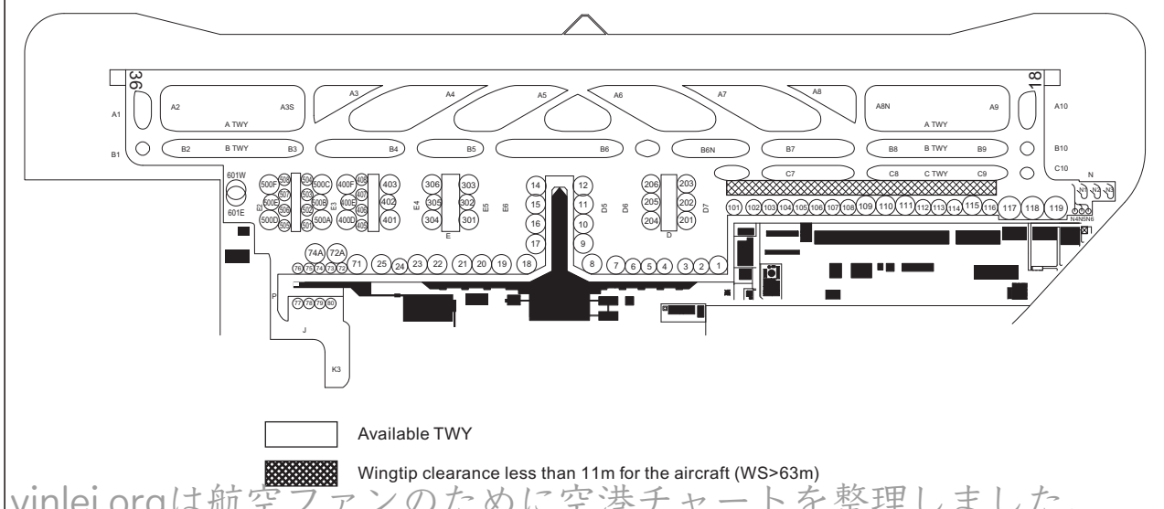
Taxiway routes available to the aircraft (WS=<65m)
