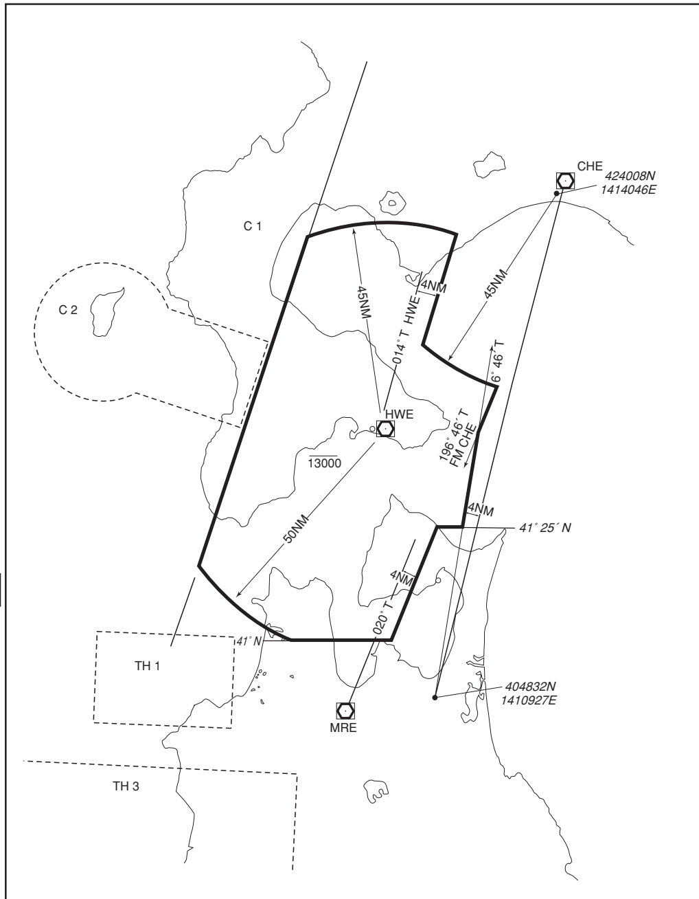
函館進入管制区 Hakodate Approach Control Area
